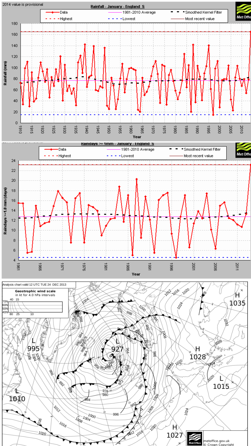
Figure 4: Surface pressure chart for 12z, 24 th December showing the formation of an intense depression to the north of Scotland.
